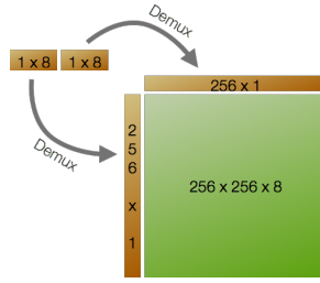
Fig. 12. Two Dimensional Demux
