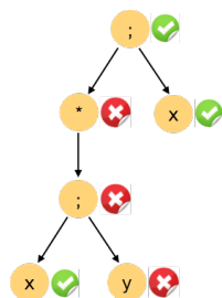
Fig. 4. Match-Annotated Regular Expression
